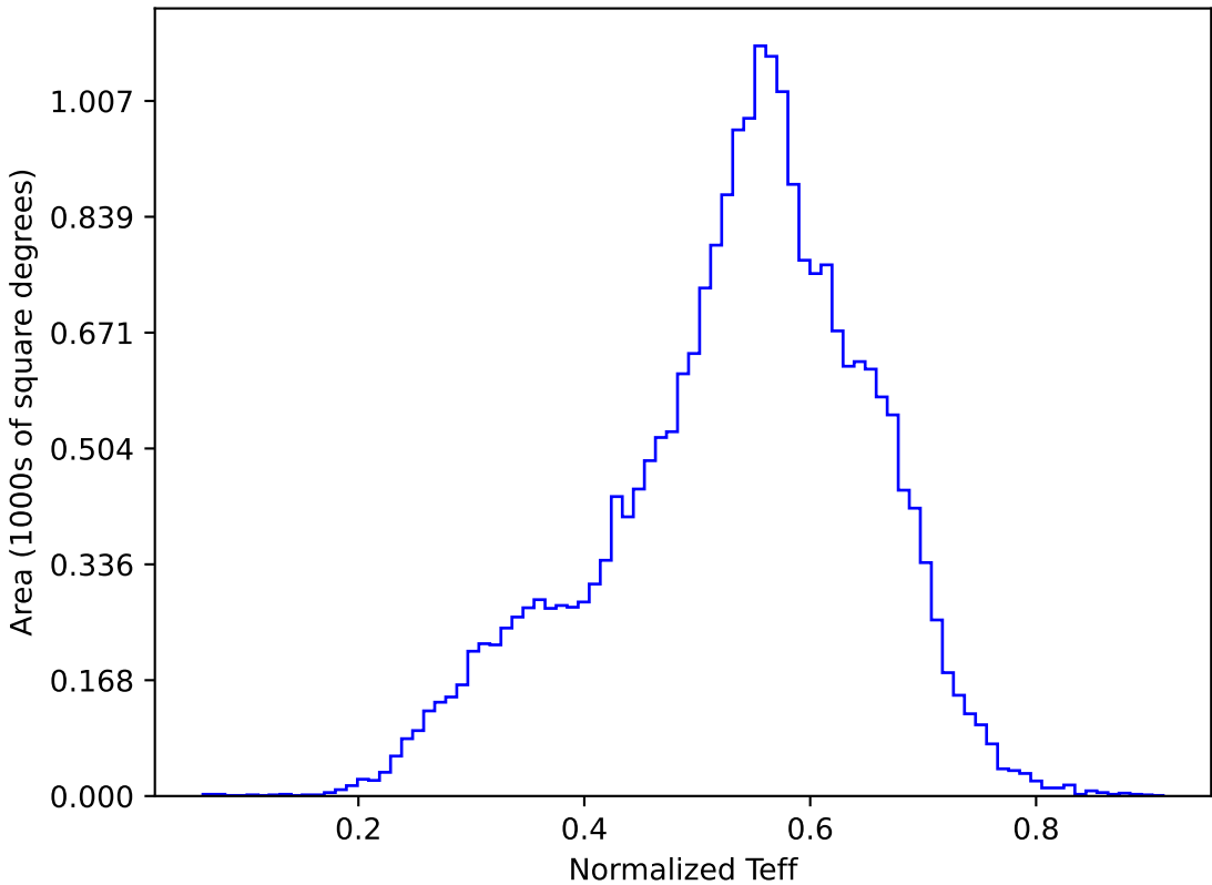
too_elab_r32_d3_gz_v3.4_10yrs All sky y band: Normalized Teff
