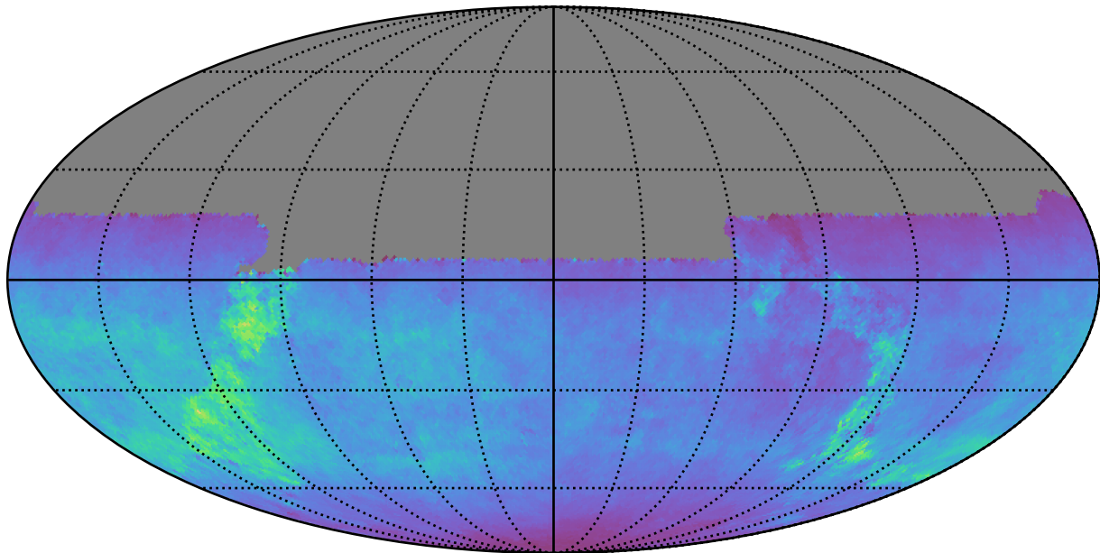
too_elab_r32_d3_gz_v3.4_10yrs All sky u band: Normalized Teff
