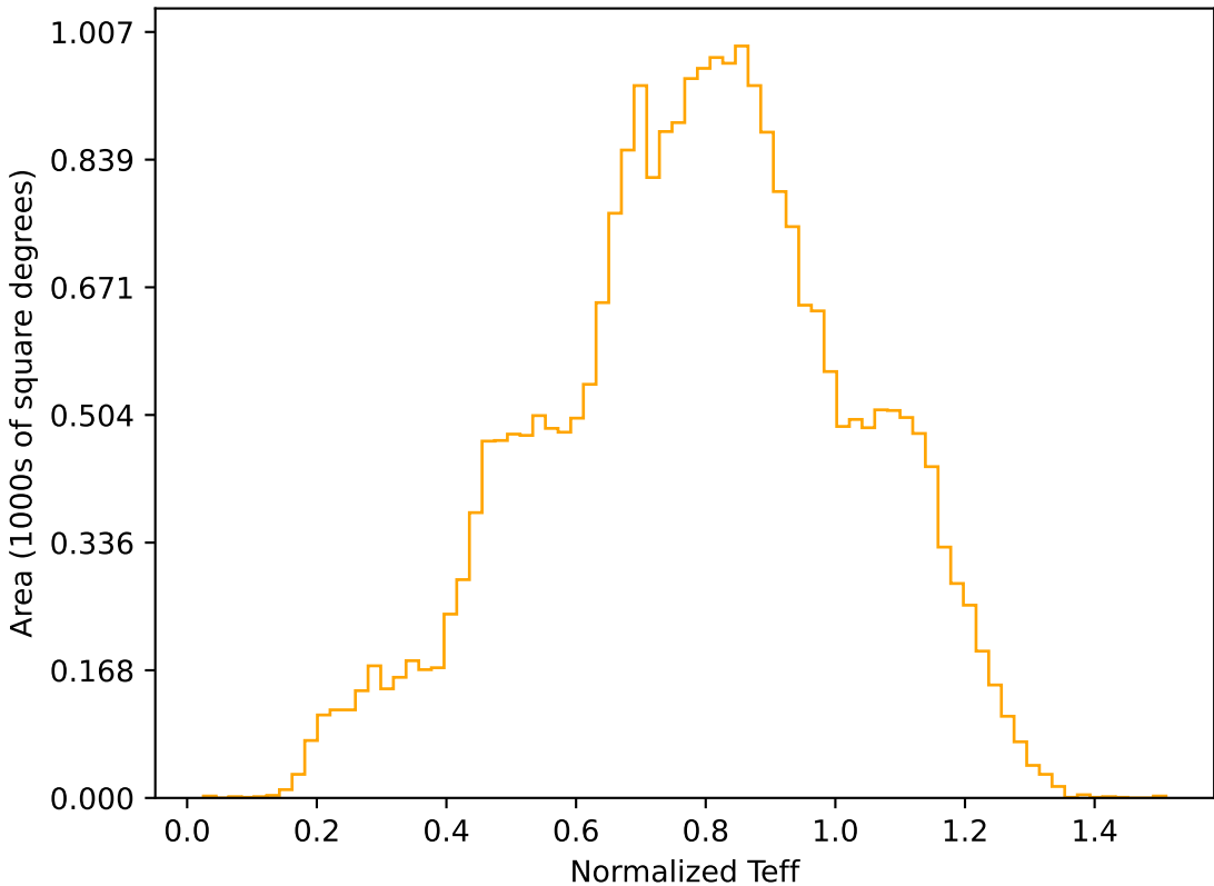
too_elab_r32_d3_gz_v3.4_10yrs All sky r band: Normalized Teff
