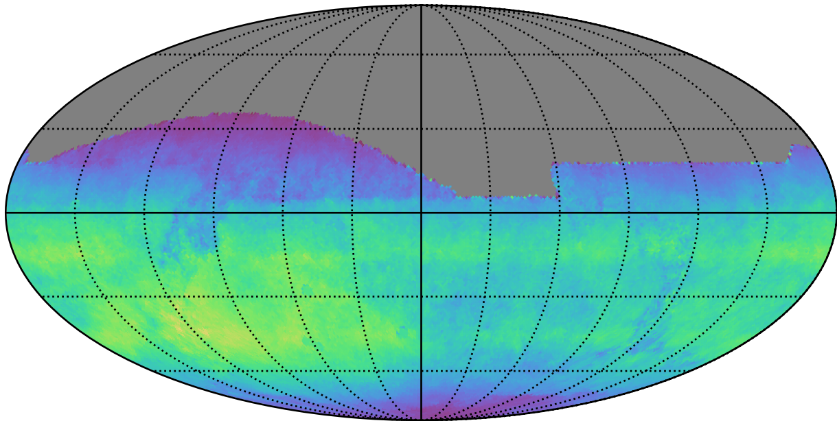
too_elab_r32_d3_gz_v3.4_10yrs All sky i band: Normalized Teff
