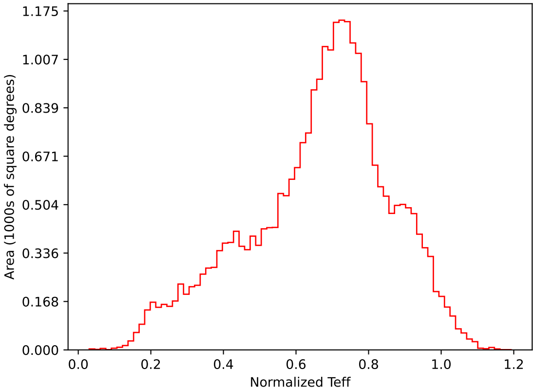
too_elab_r32_d3_gz_v3.4_10yrs All sky i band: Normalized Teff
