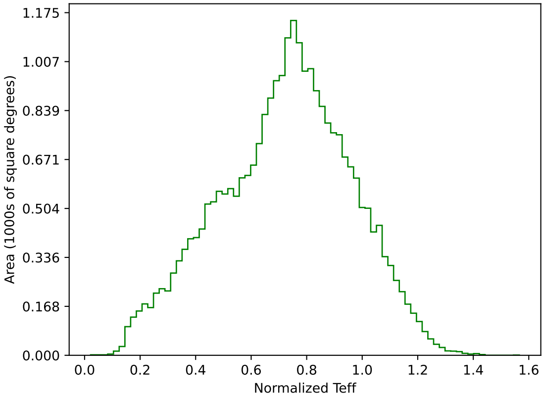
too_elab_r32_d3_gz_v3.4_10yrs All sky g band: Normalized Teff
