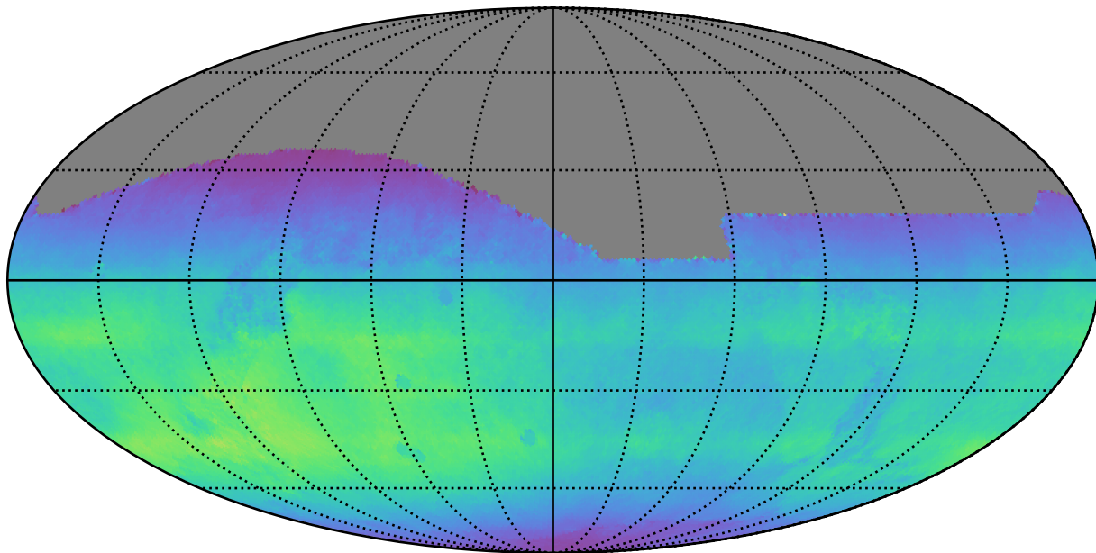
too_elab_r32_d3_gz_v3.4_10yrs All sky all bands: Normalized Teff
