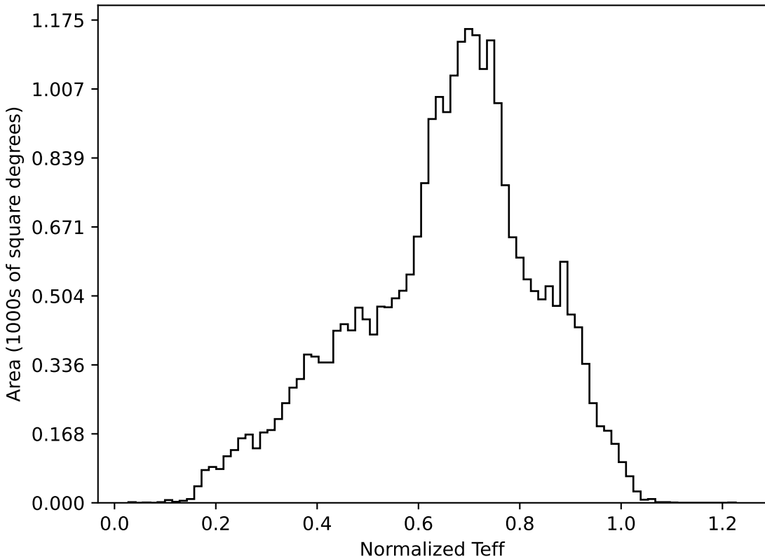
too_elab_r32_d3_gz_v3.4_10yrs All sky all bands: Normalized Teff
