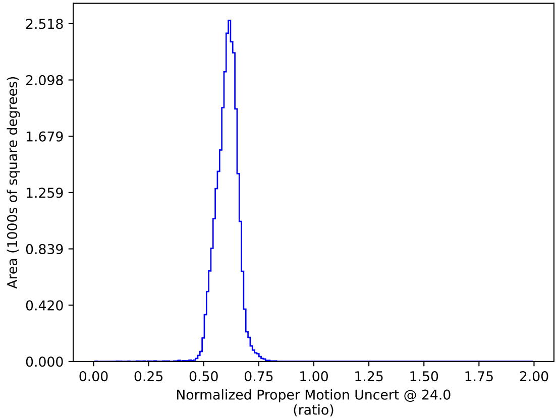
too_elab_r32_d3_gz_v3.4_10yrs All sky: Normalized Proper Motion Uncert @ 24.0
