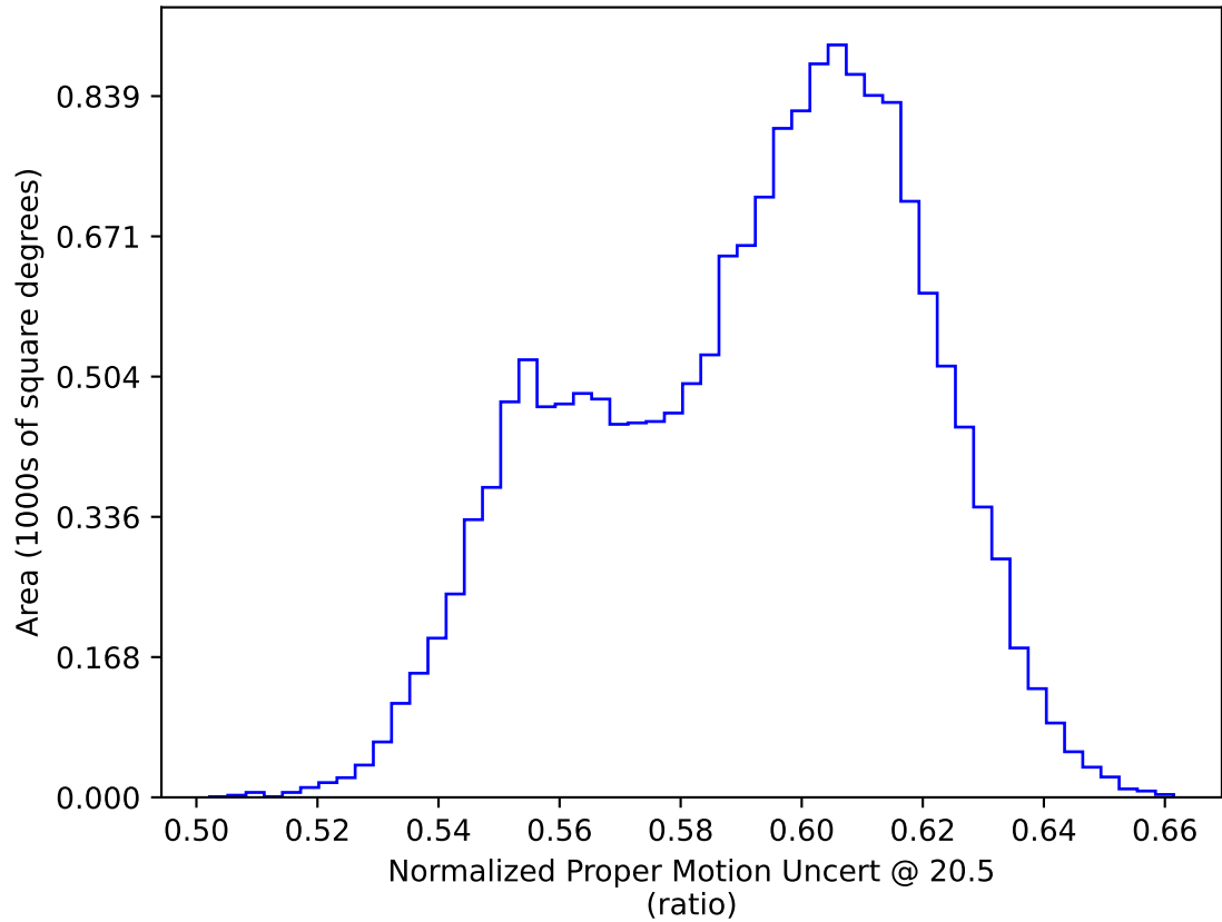
too_elab_r32_d3_gz_v3.4_10yrs WFD: Normalized Proper Motion Uncert @ 20.5
