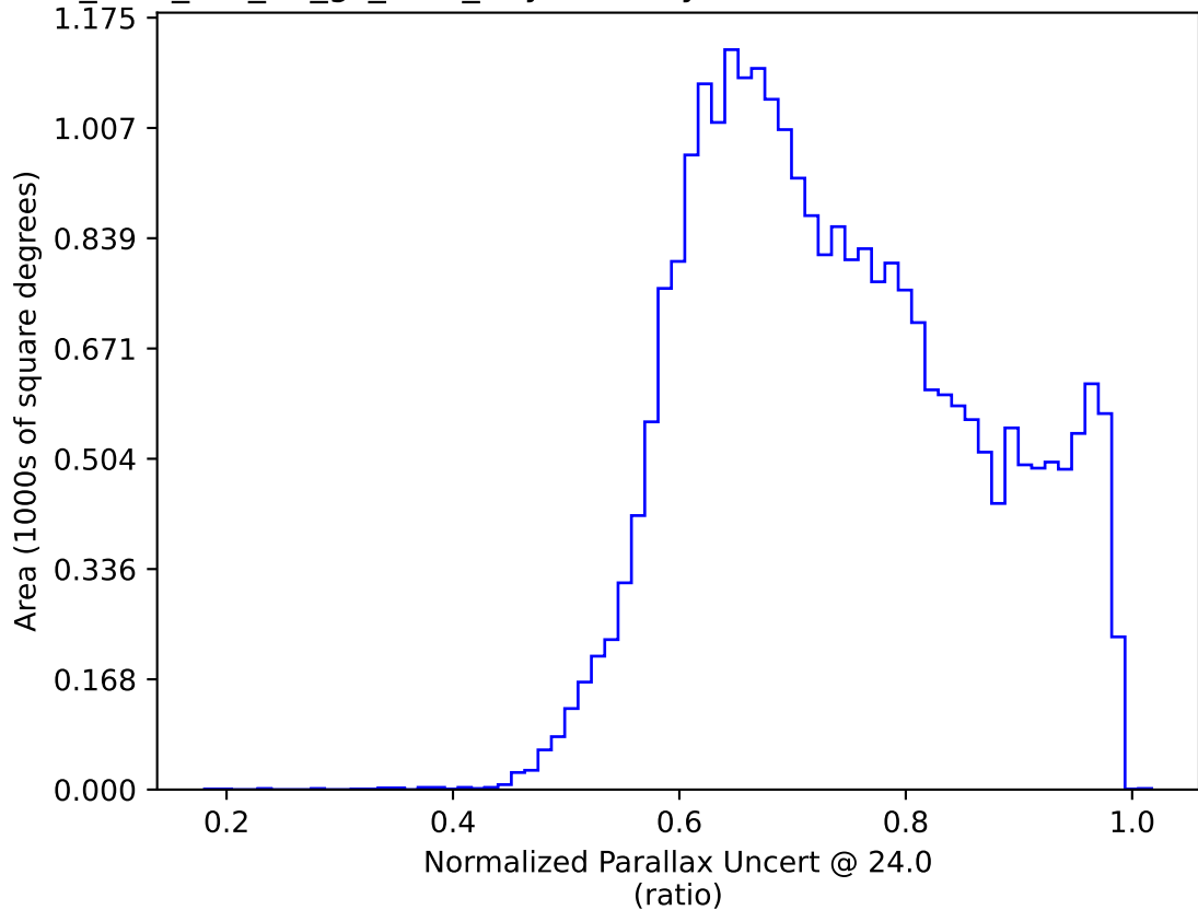
too_elab_r32_d3_gz_v3.4_10yrs All sky: Normalized Parallax Uncert @ 24.0
