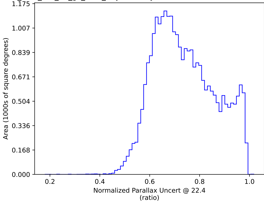
too_elab_r32_d3_gz_v3.4_10yrs All sky: Normalized Parallax Uncert @ 22.4
