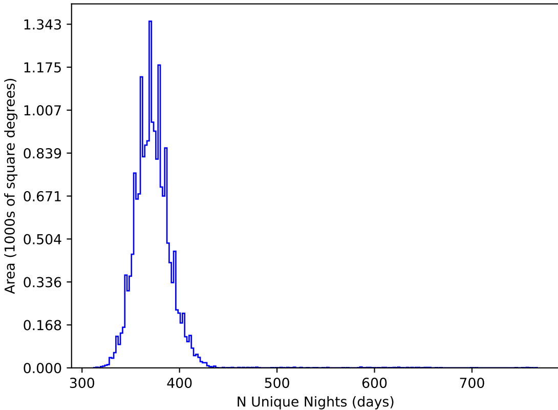
too_elab_r32_d3_gz_v3.4_10yrs WFD all bands: N Unique Nights
