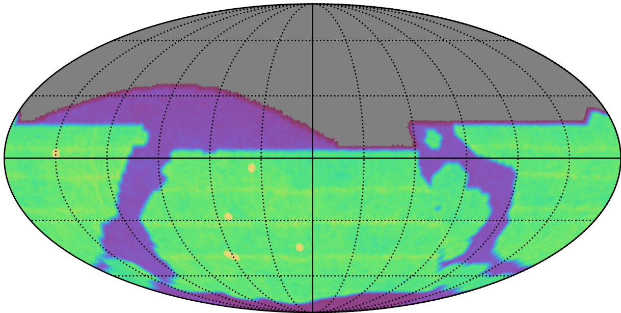
too_elab_r32_d3_gz_v3.4_10yrs All sky all bands: N Unique Nights
