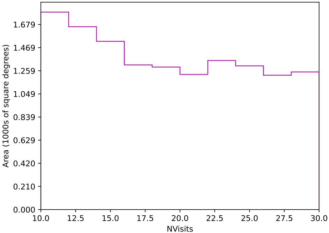
too_elab_r32_d3_gz_v3.4_10yrs Yr 3-4 z band: NVisits
