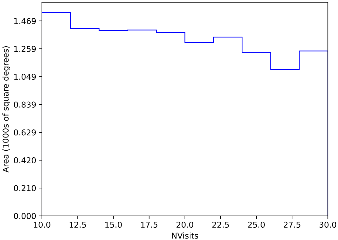
too_elab_r32_d3_gz_v3.4_10yrs Yr 3-4 y band: NVisits
