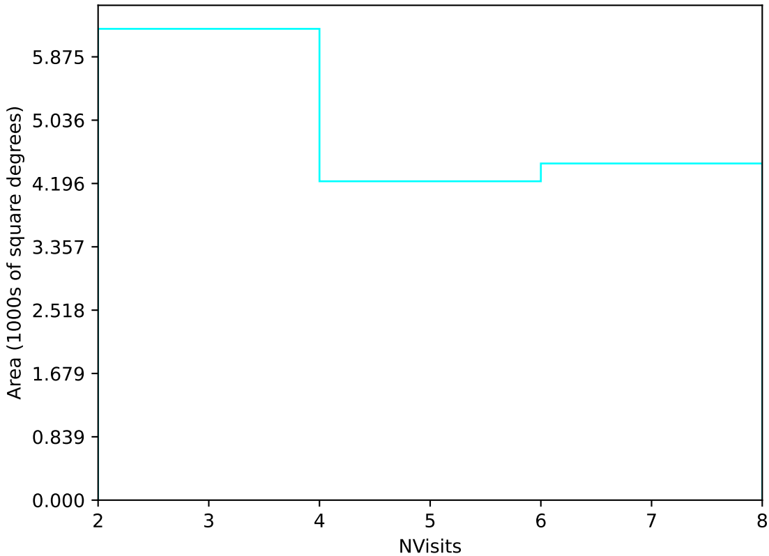
too_elab_r32_d3_gz_v3.4_10yrs Yr 3-4 u band: NVisits
