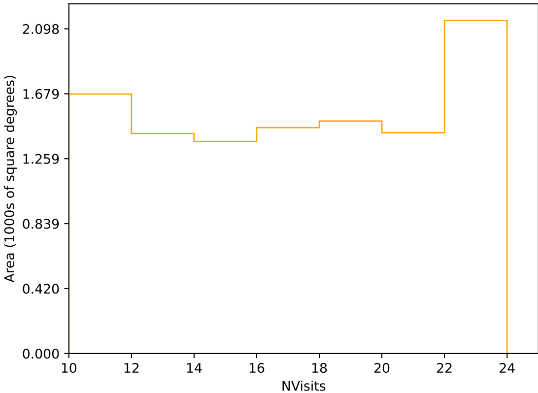
too_elab_r32_d3_gz_v3.4_10yrs Yr 3-4 r band: NVisits
