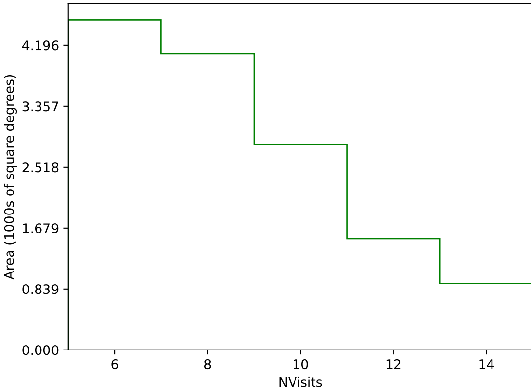
too_elab_r32_d3_gz_v3.4_10yrs Yr 3-4 g band: NVisits
