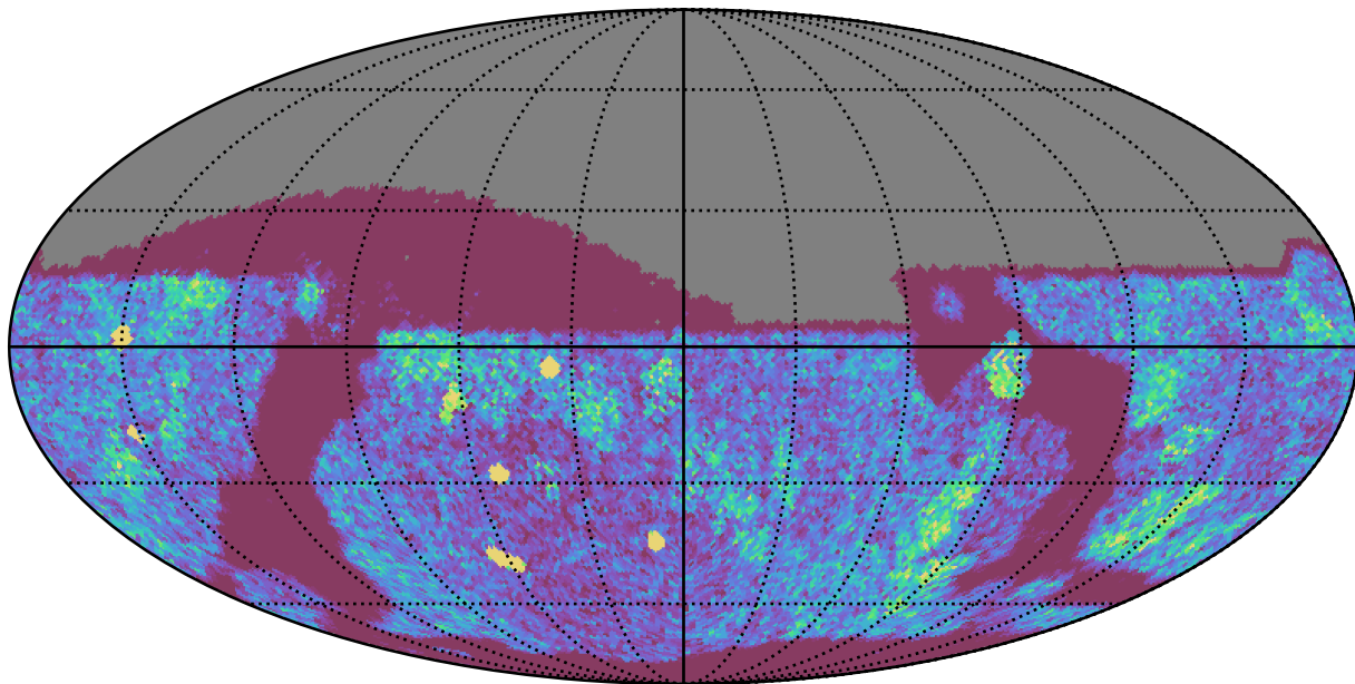
too_elab_r32_d3_gz_v3.4_10yrs Yr 1 z band: NVisits
