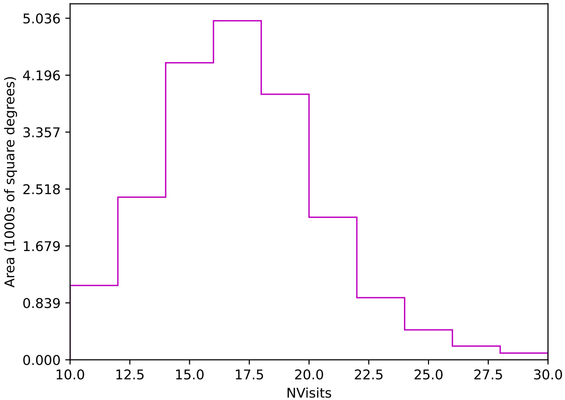
too_elab_r32_d3_gz_v3.4_10yrs Yr 1 z band: NVisits
