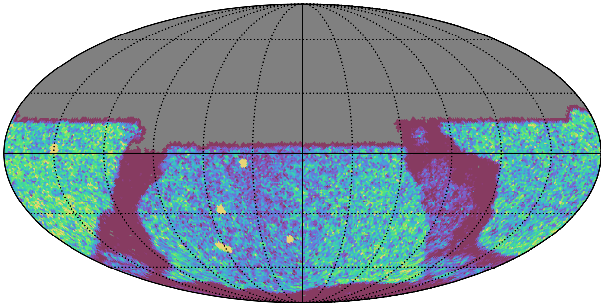
too_elab_r32_d3_gz_v3.4_10yrs Yr 1 y band: NVisits
