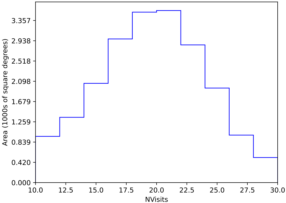
too_elab_r32_d3_gz_v3.4_10yrs Yr 1 y band: NVisits
