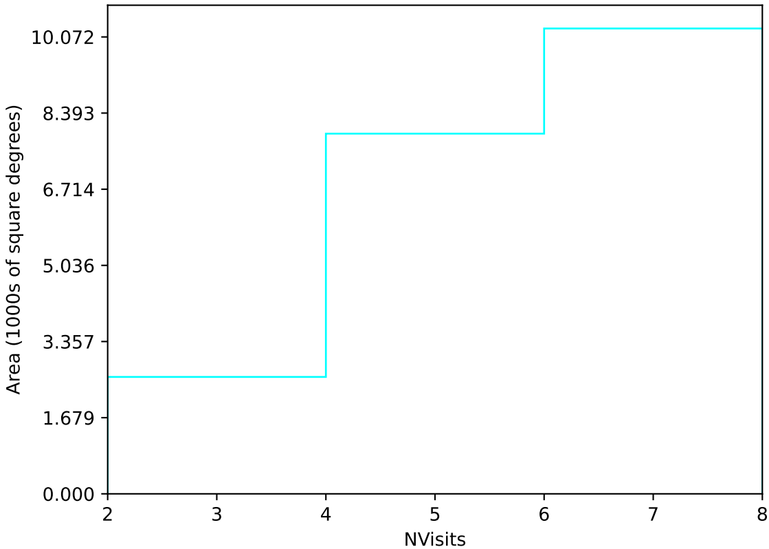
too_elab_r32_d3_gz_v3.4_10yrs Yr 1 u band: NVisits
