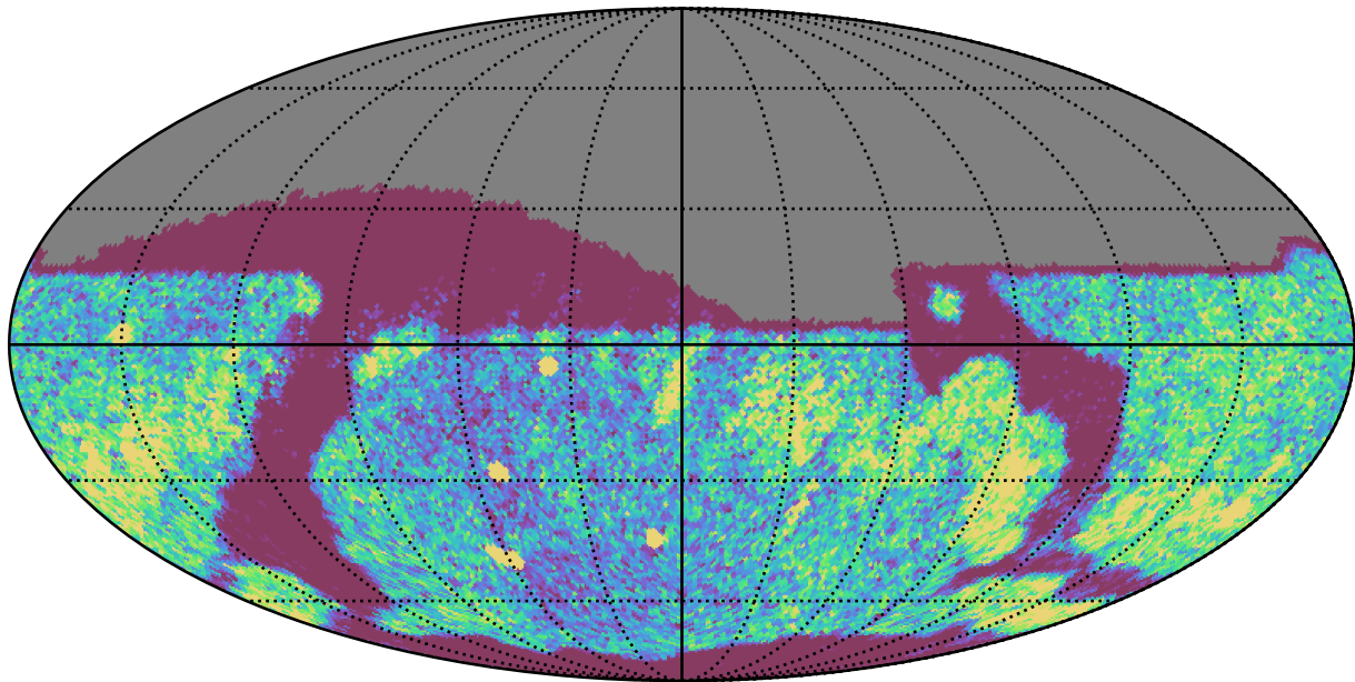
too_elab_r32_d3_gz_v3.4_10yrs Yr 1 r band: NVisits
