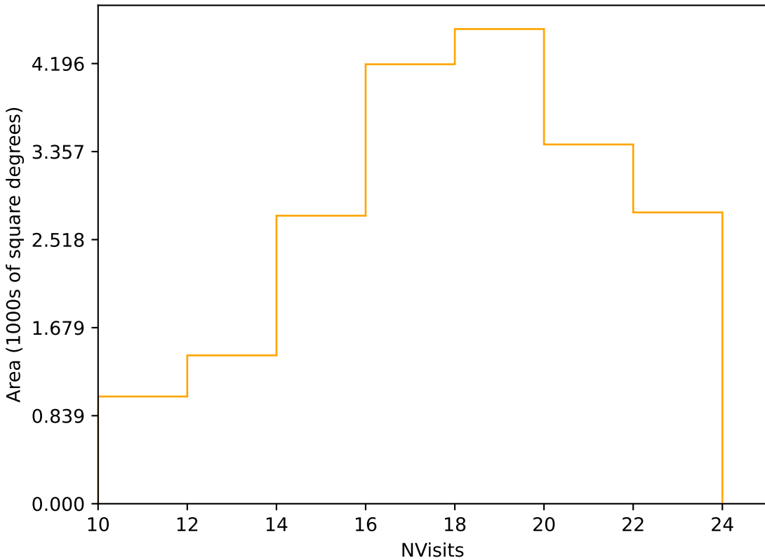
too_elab_r32_d3_gz_v3.4_10yrs Yr 1 r band: NVisits
