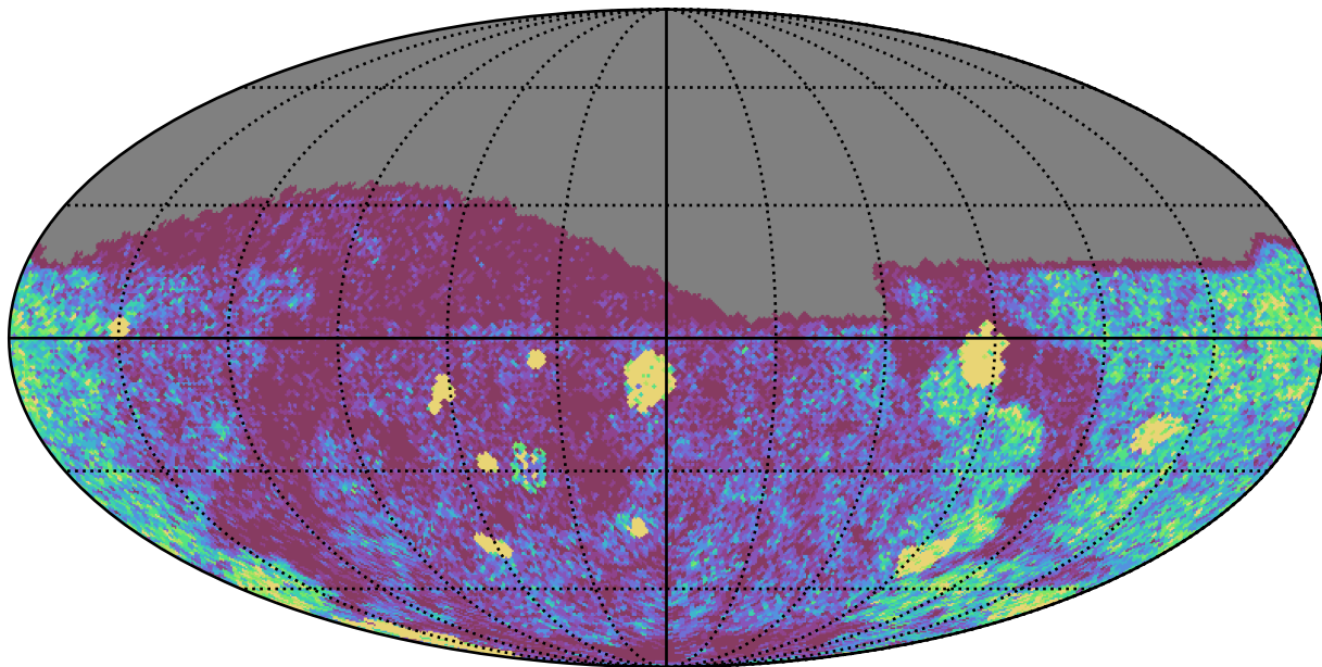
too_elab_r32_d3_gz_v3.4_10yrs Yr 1 g band: NVisits
