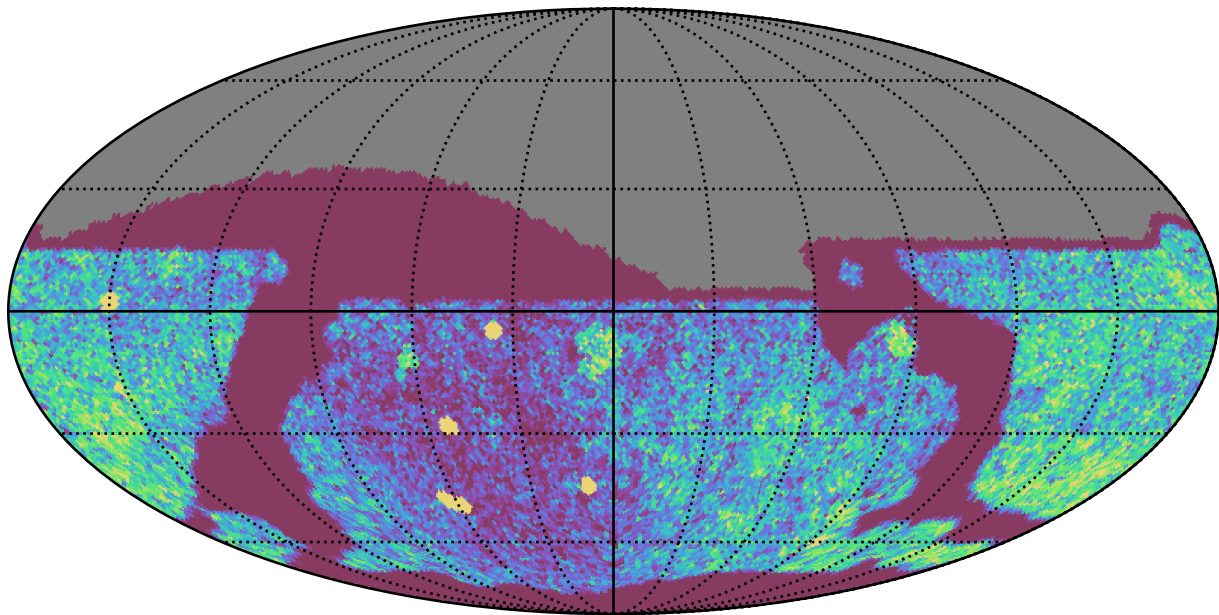
too_elab_r32_d3_gz_v3.4_10yrs Yr 1 all bands: NVisits
