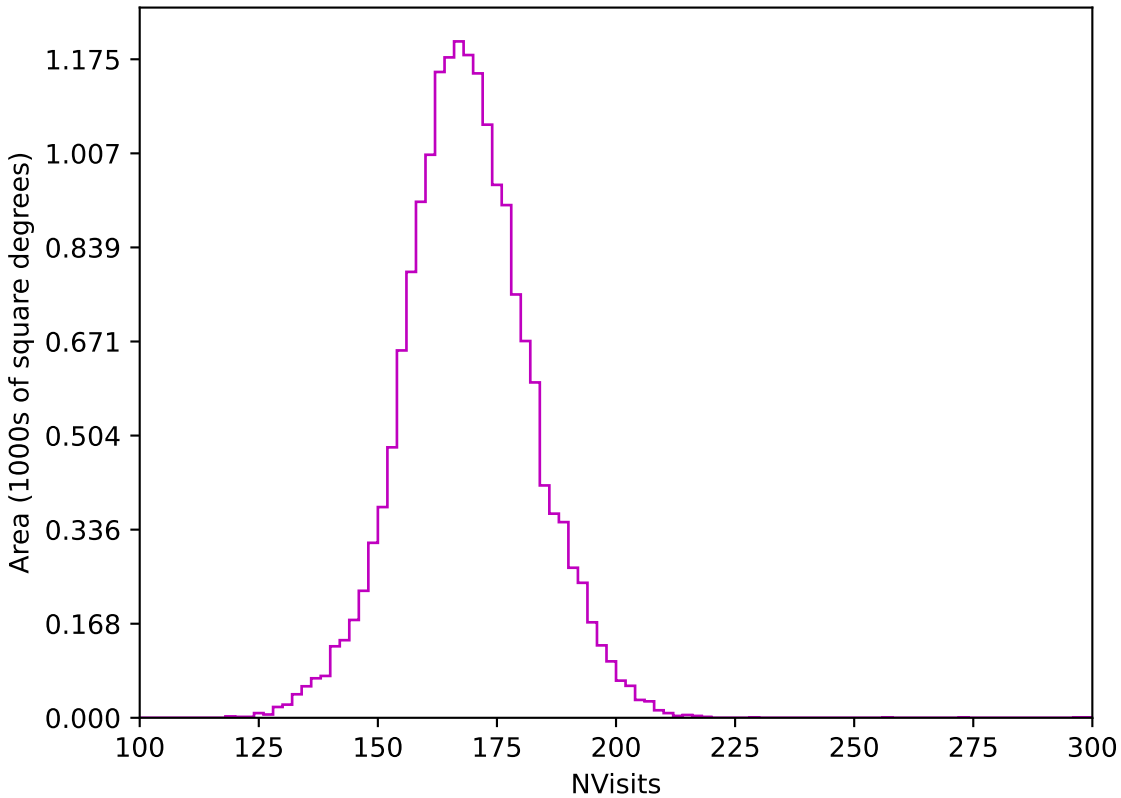
too_elab_r32_d3_gz_v3.4_10yrs WFD z band: NVisits
