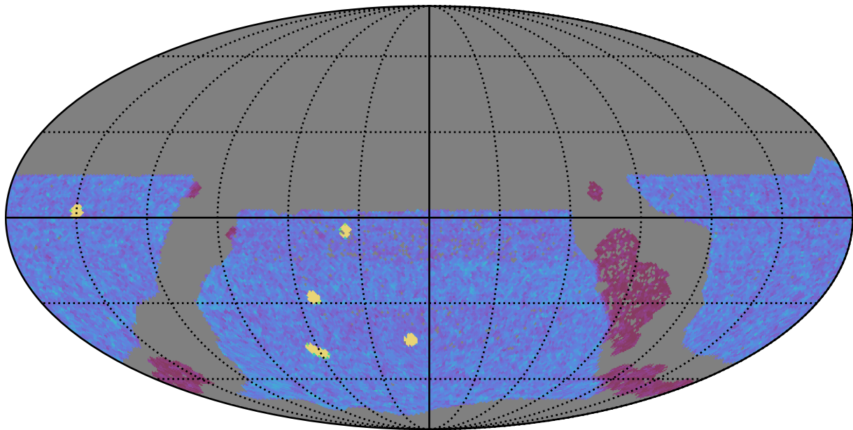
too_elab_r32_d3_gz_v3.4_10yrs WFD y band: NVisits
