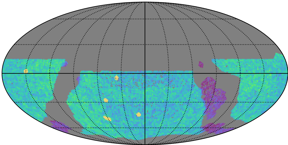
too_elab_r32_d3_gz_v3.4_10yrs WFD u band: NVisits
