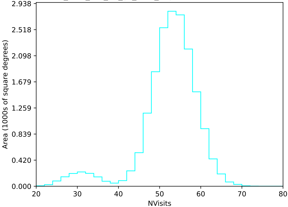
too_elab_r32_d3_gz_v3.4_10yrs WFD u band: NVisits
