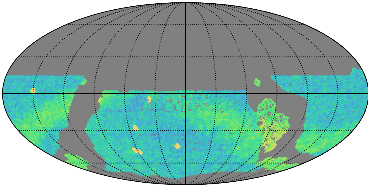
too_elab_r32_d3_gz_v3.4_10yrs WFD r band: NVisits
