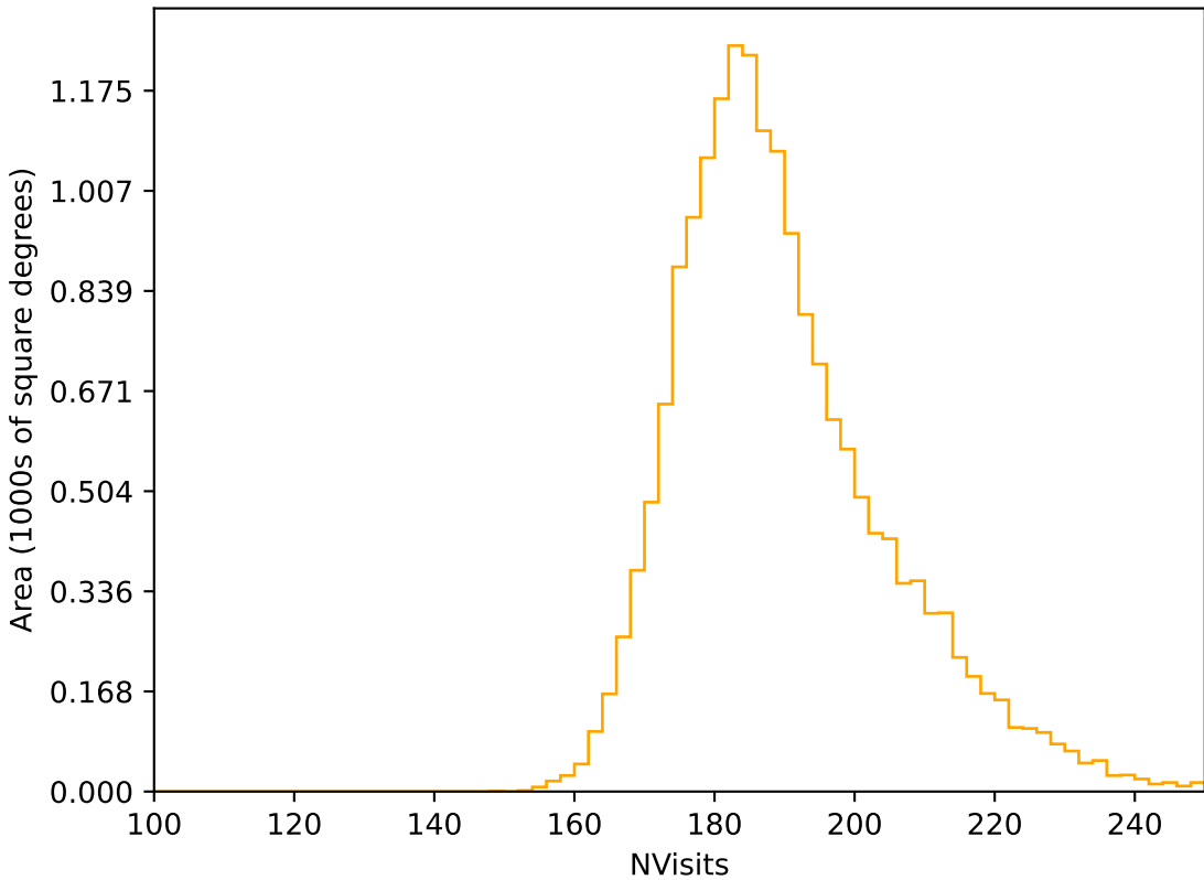
too_elab_r32_d3_gz_v3.4_10yrs WFD r band: NVisits
