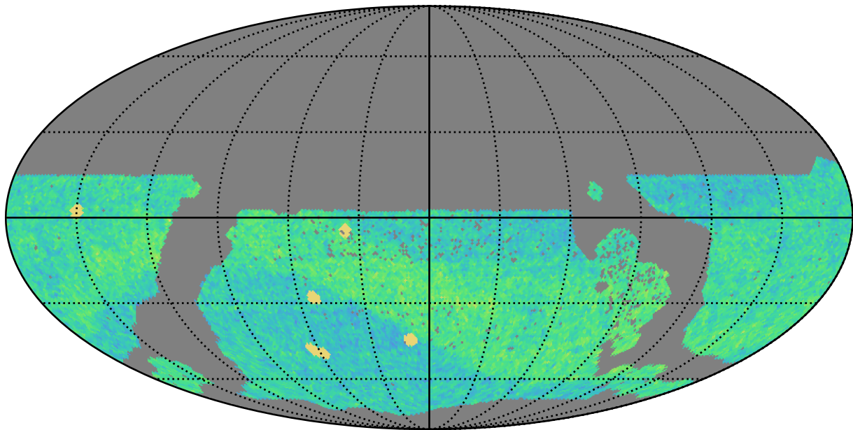
too_elab_r32_d3_gz_v3.4_10yrs WFD i band: NVisits
