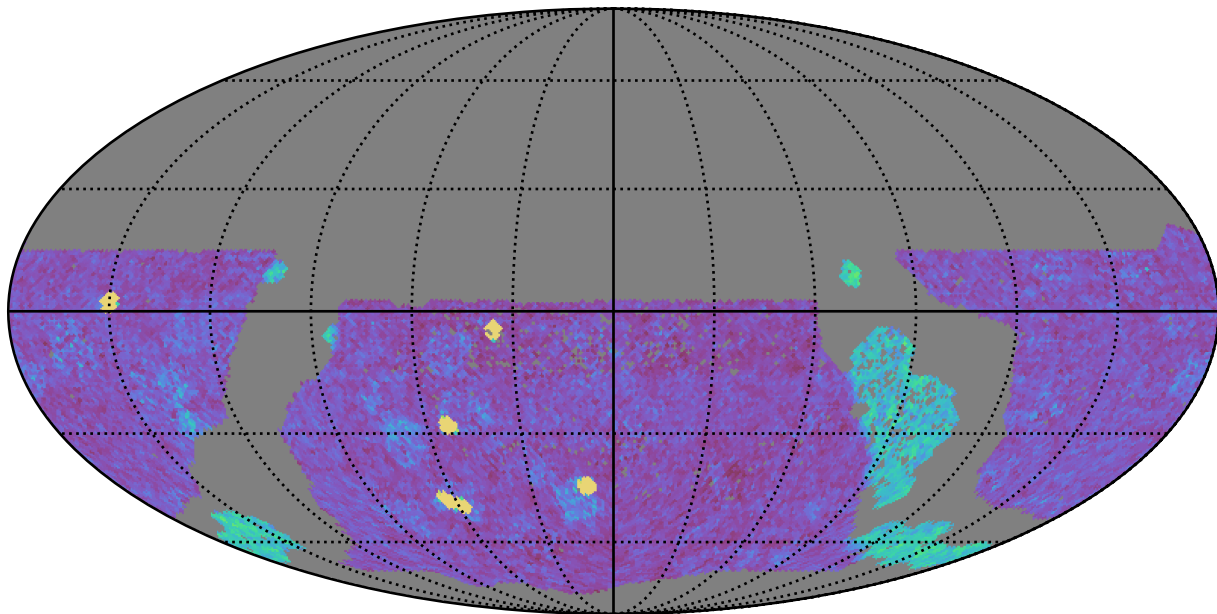
too_elab_r32_d3_gz_v3.4_10yrs WFD g band: NVisits
