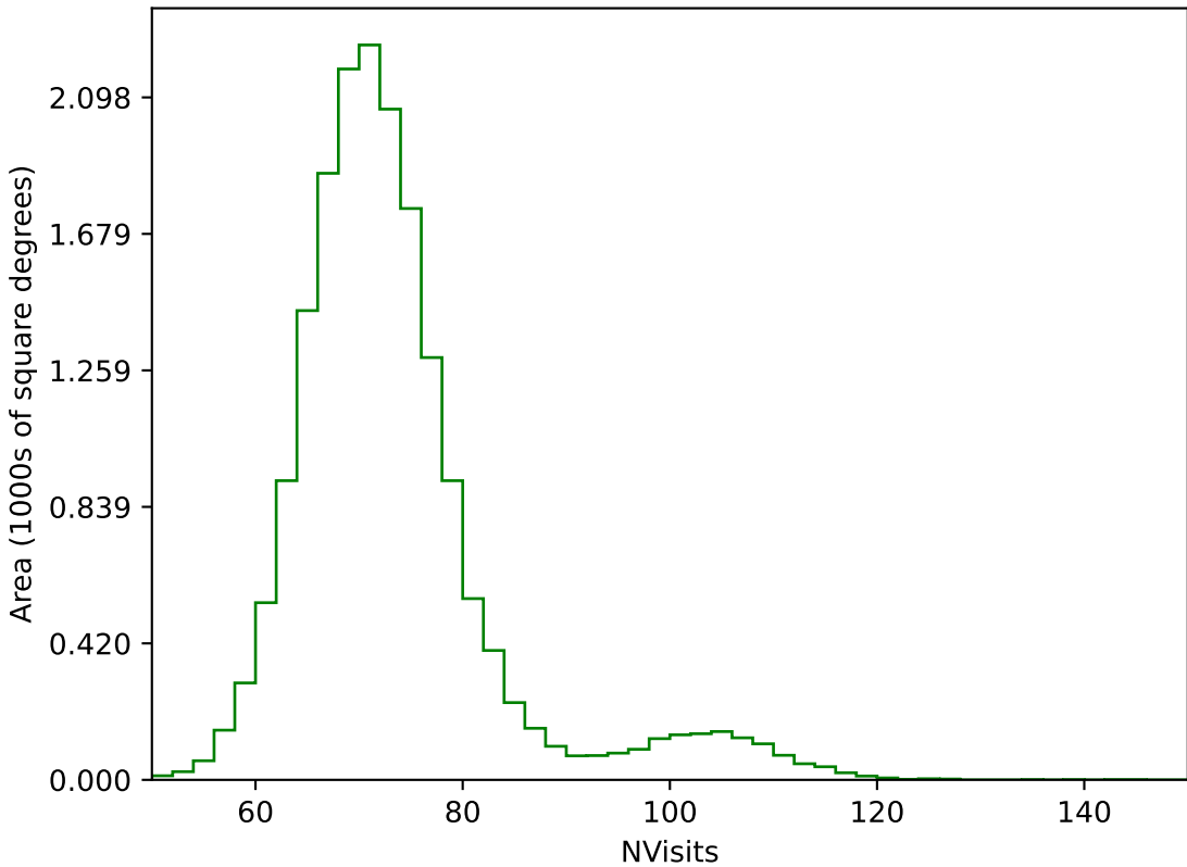
too_elab_r32_d3_gz_v3.4_10yrs WFD g band: NVisits
