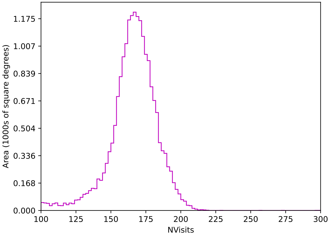
too_elab_r32_d3_gz_v3.4_10yrs All sky z band: NVisits
