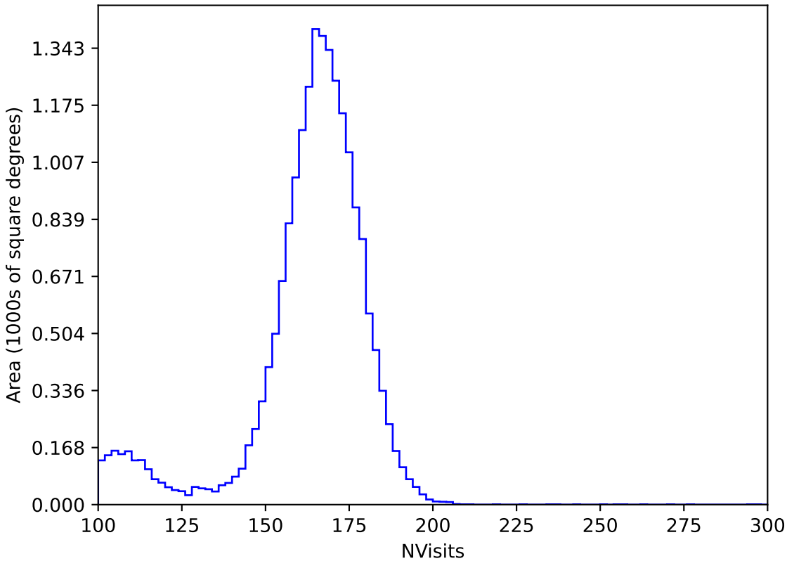
too_elab_r32_d3_gz_v3.4_10yrs All sky y band: NVisits
