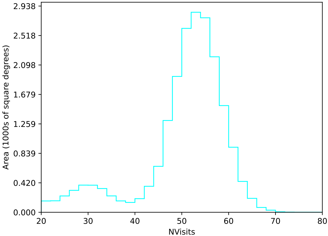
too_elab_r32_d3_gz_v3.4_10yrs All sky u band: NVisits
