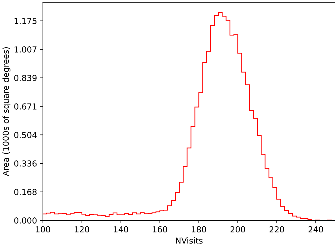
too_elab_r32_d3_gz_v3.4_10yrs All sky i band: NVisits
