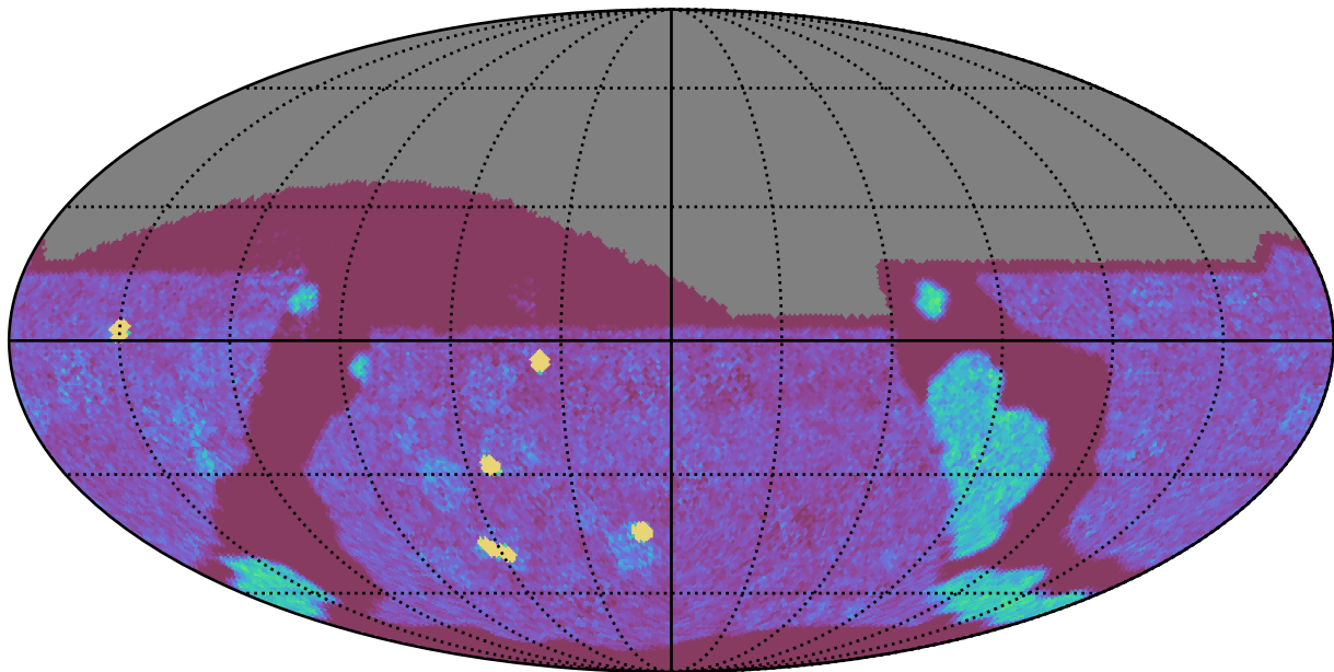
too_elab_r32_d3_gz_v3.4_10yrs All sky g band: NVisits
