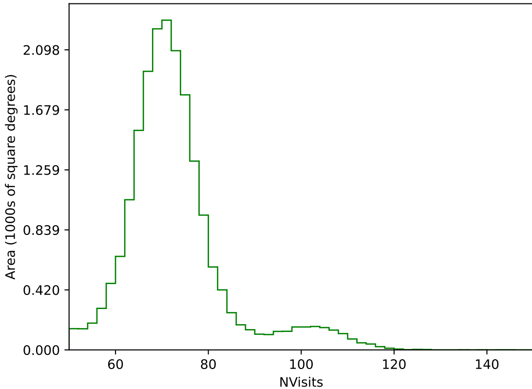
too_elab_r32_d3_gz_v3.4_10yrs All sky g band: NVisits
