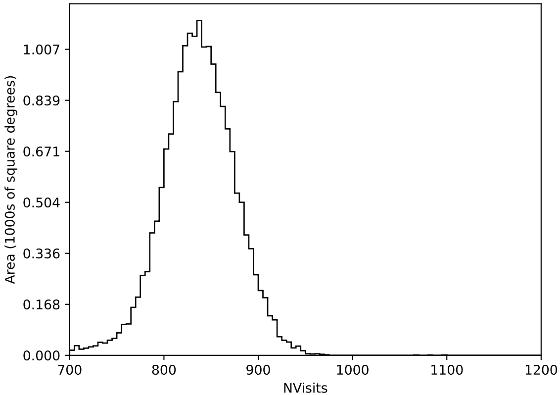
too_elab_r32_d3_gz_v3.4_10yrs All sky all bands: NVisits
