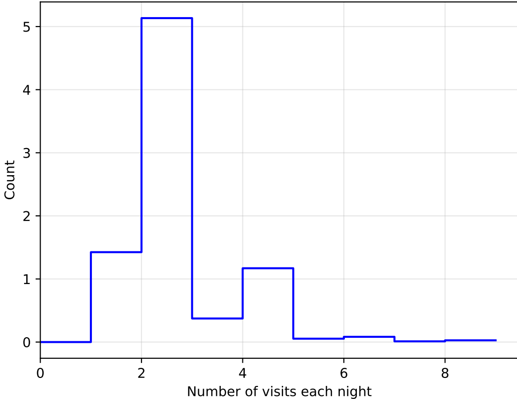
too_elab_r32_d3_gz_v3.4_10yrs WFD: NVisitsPerNight
