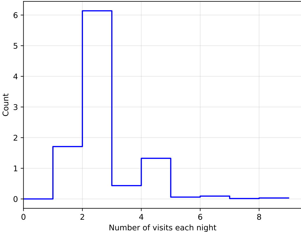
too_elab_r32_d3_gz_v3.4_10yrs All sky: NVisitsPerNight
