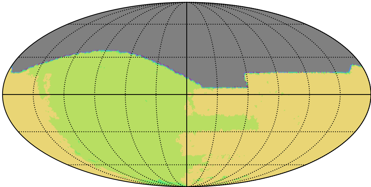
too_elab_r32_d3_gz_v3.4_10yrs All sky all bands: NSeasons
