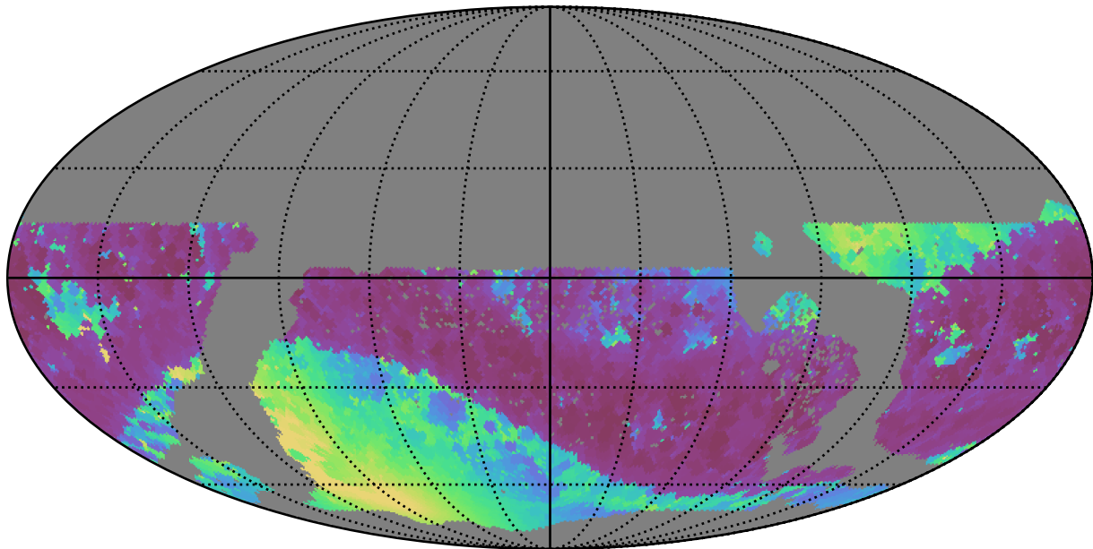
too_elab_r32_d3_gz_v3.4_10yrs WFD z band: Min solarElong
