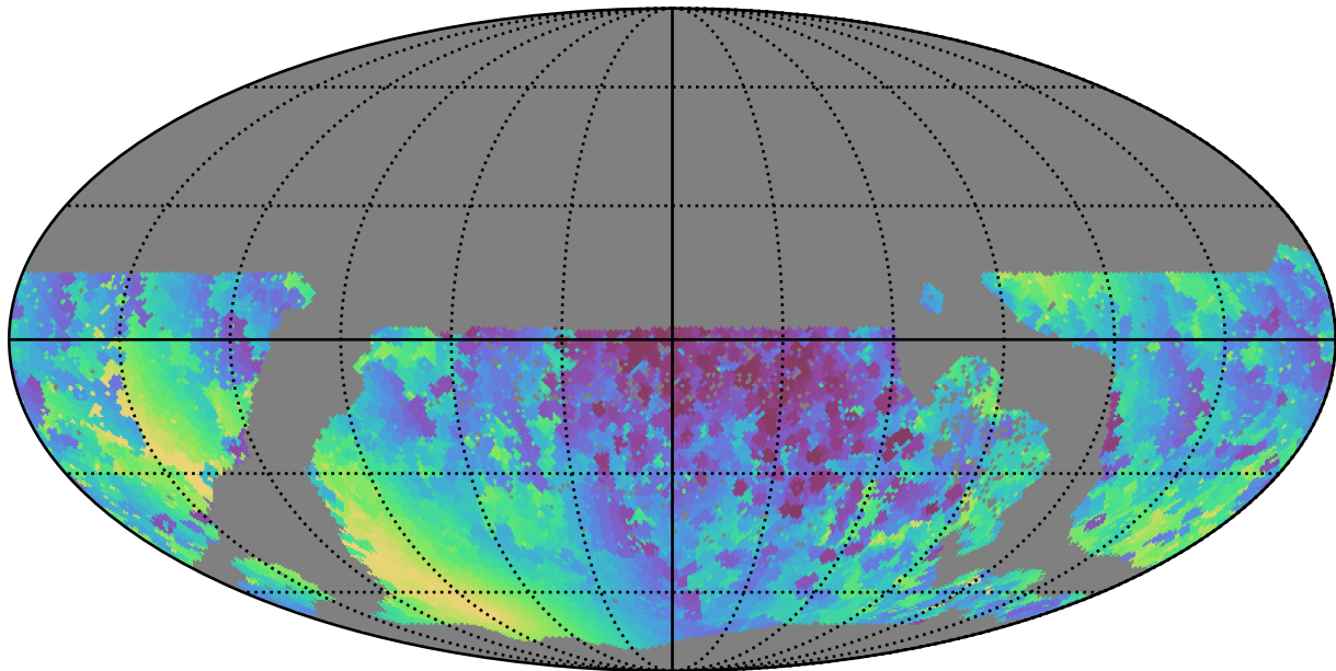
too_elab_r32_d3_gz_v3.4_10yrs WFD y band: Min solarElong
