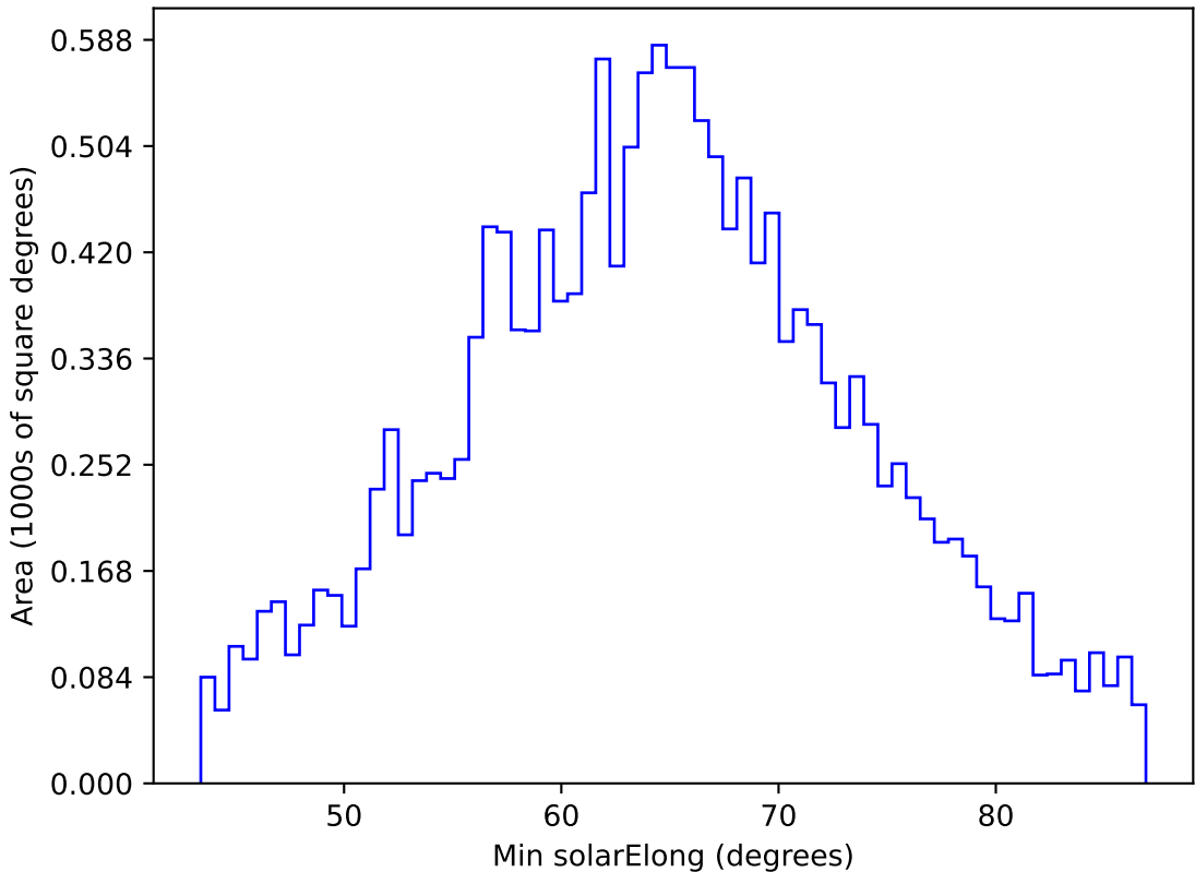
too_elab_r32_d3_gz_v3.4_10yrs WFD y band: Min solarElong
